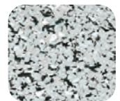
Steel
